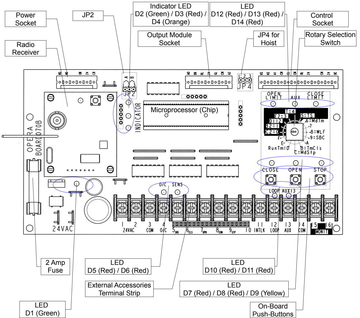
Figure 30 - Electronic Control Board – BOARD 070M
