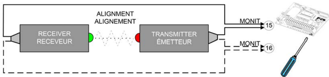
Figure 13 - PHOTO 061/062/064/070 Connection
