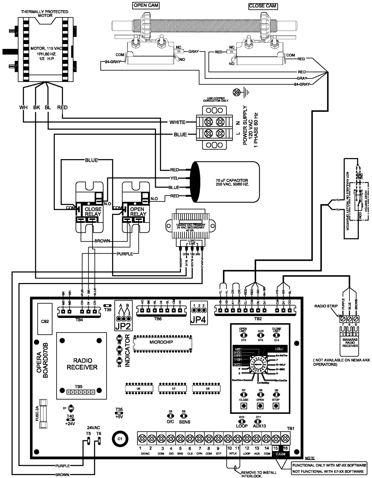
Figure 32 - EDWG11070R6801
