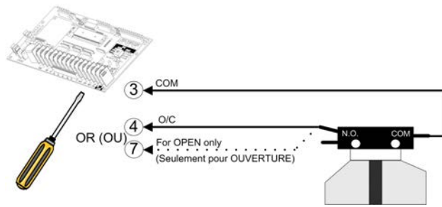
Figure 26 - PULLCORD 001 / 003 / 004 / 007
