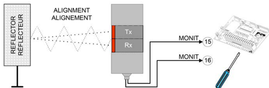
Figure 14 - PHOTO 065 Connection
