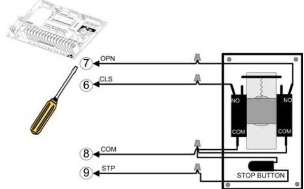
Figure 28 - KEYSWITCH 019
