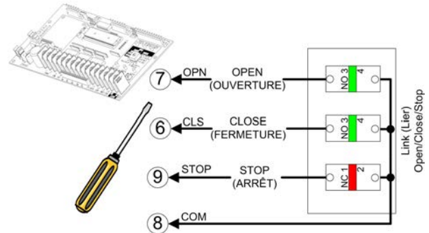
Figure 8 - STATION 041 / 049 / 056 / 076 / 078 3-PBS Open / Close / Stop
