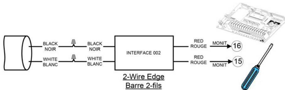
Figure 16 - SENSEEDGE 044UM and INTERFACE 002 Connection
