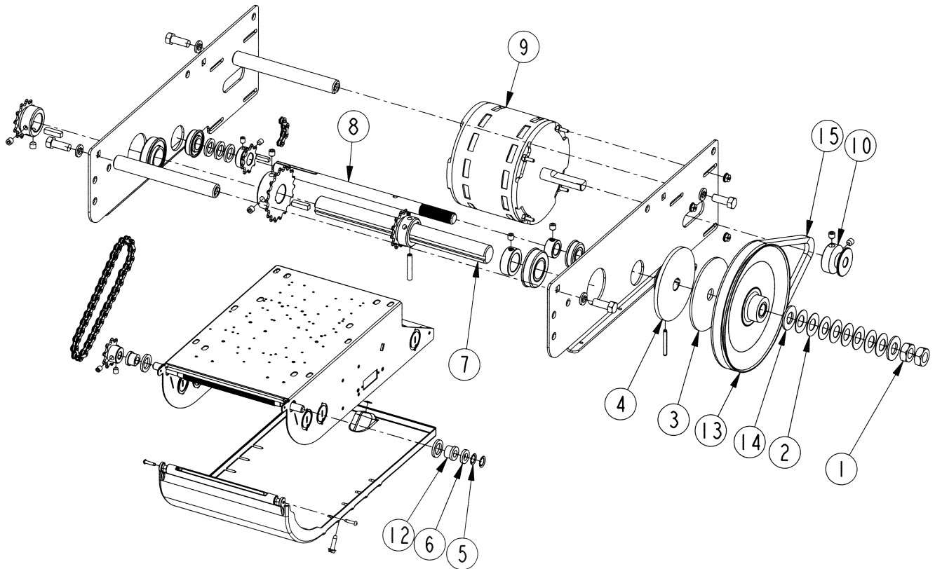
Figure 35 - OMT Mechanical Exploded View
