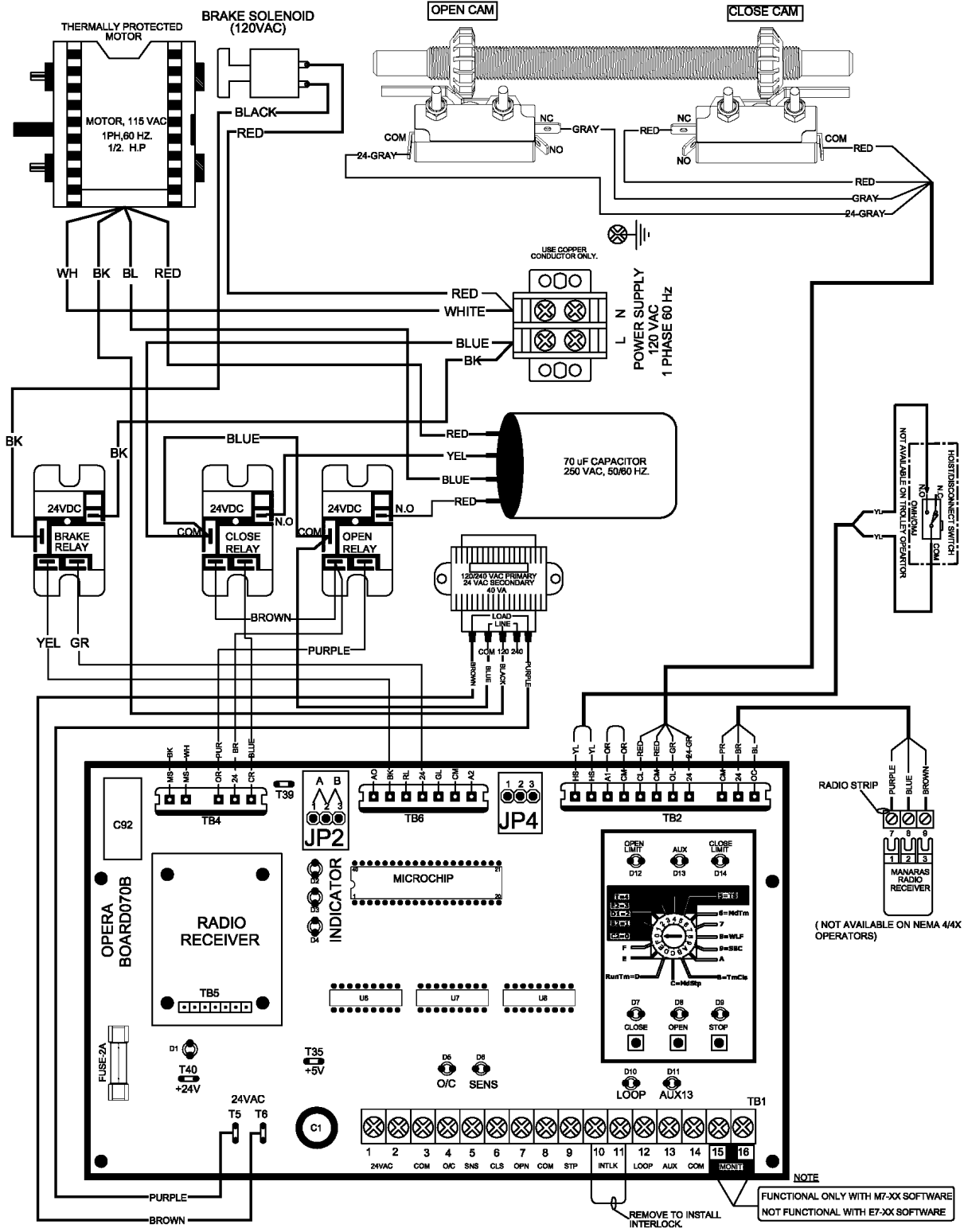
Figure 33 - EDWG11070R6802
