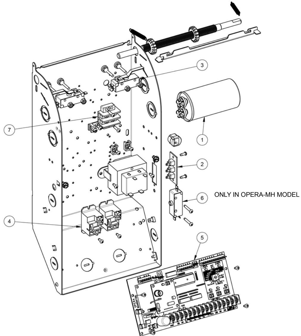
Figure 36 - Opera-MH, Opera-MJ and OMT Control Box with BOARD 070M
