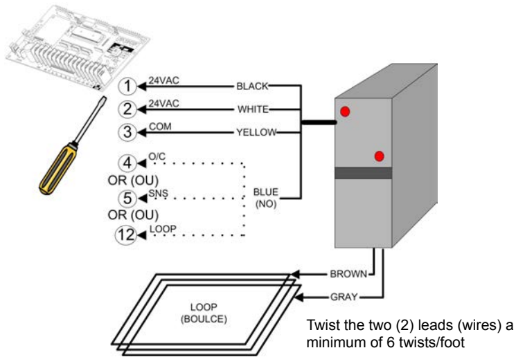
Figure 29 - Vehicle Loop Detector
