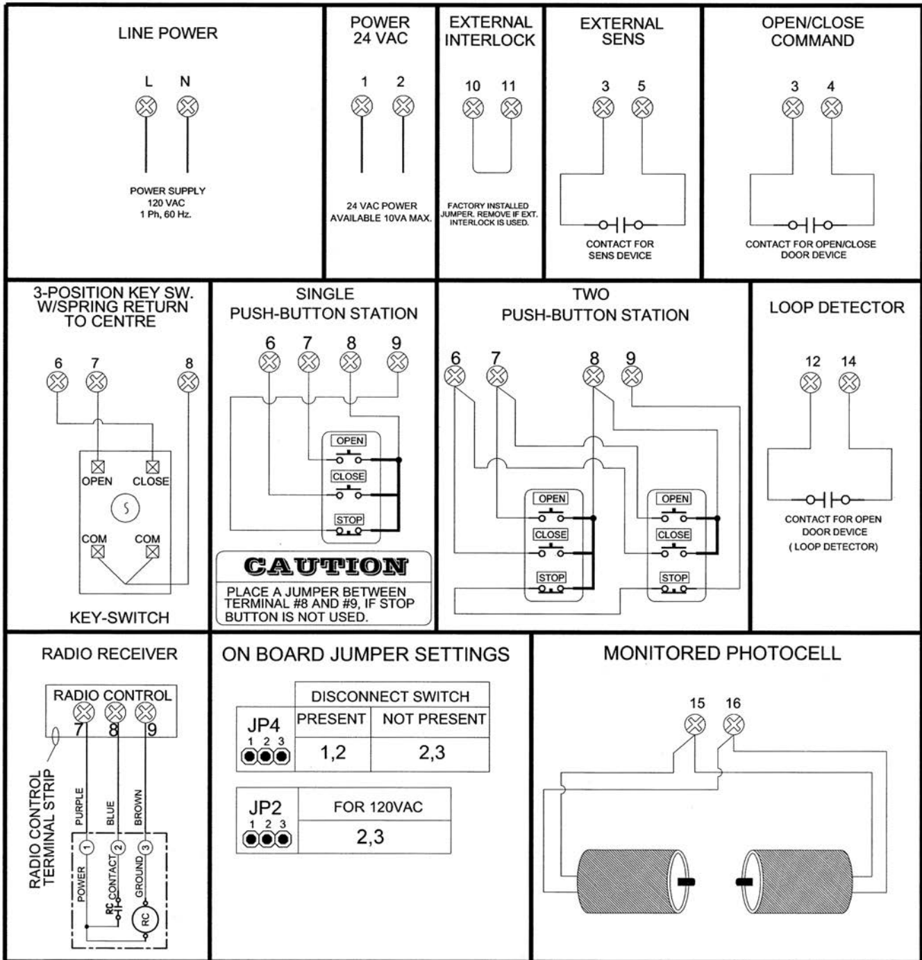
Figure 34 - External Wiring
