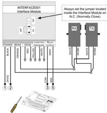
Figure 17 - PHOTO 008A/B
