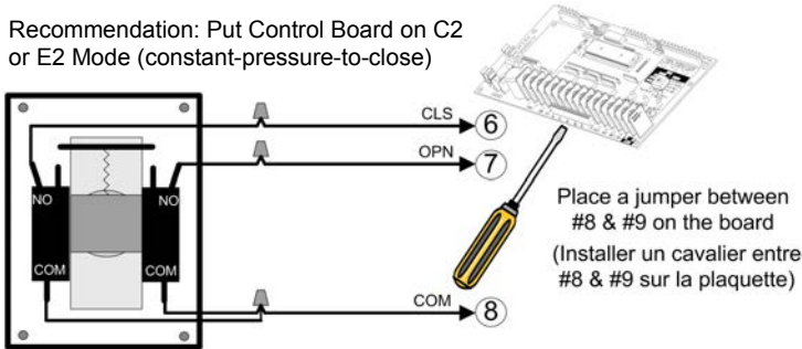
Figure 27 - KEYSWITCH 010 / 015
